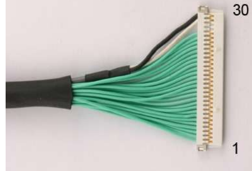
Hirose DF19-30S-1C
