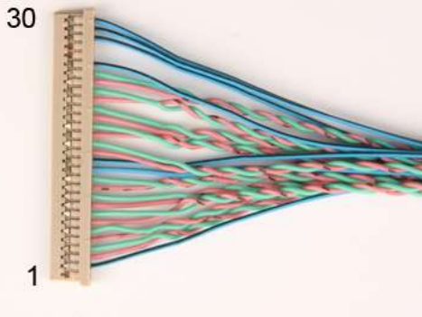
Hirose DF14-30S-1,25C
