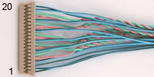
Hirose DF14-20S-1,25C
