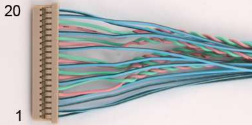
Hirose DF14-20S-1,25C
