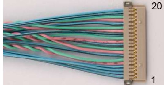
Hirose DF19-20S-1C
