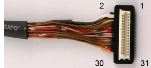
Hirose DF9-31S-1V
