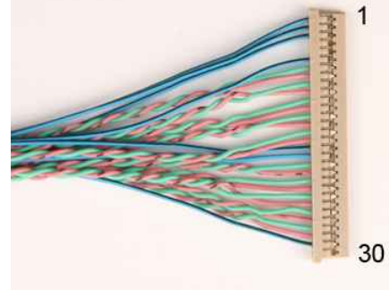
Hirose DF14-30S-1,25C
