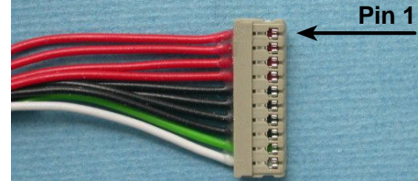
ACES 91209-01011 - 10 pin
