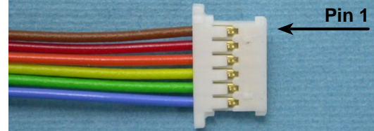
Molex 51146 - 6 Pin - 1.25 mm.
