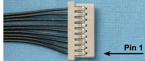
Hirose DF14-09S-1.25C
